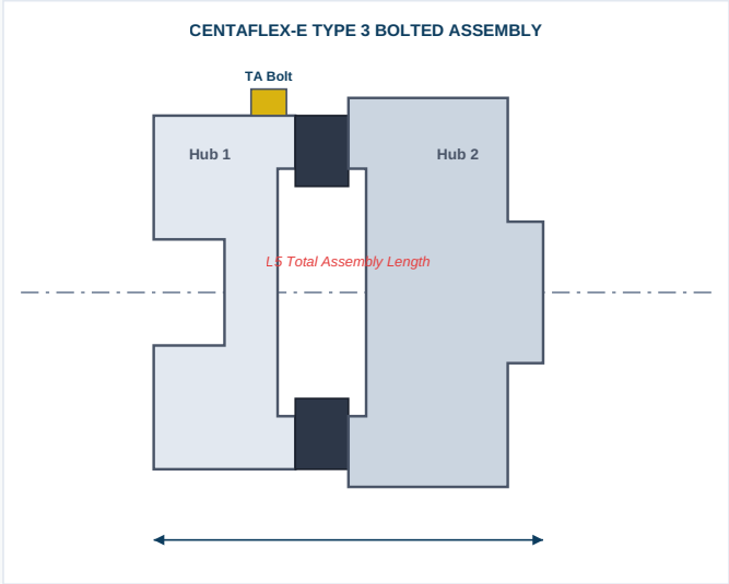
Figure 1: Sectional technical drawing highlighting the specialized clamping hardware arrangement (Part 3) and torque-locked configuration ($T_A$) of a CENTAFLEX-E Type 3 hub.
